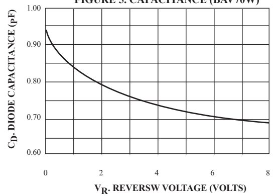
FIGURE 5. CAPACITANCE (BAV70W)
