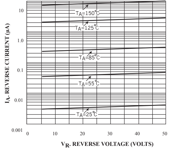
FIGURE 3. LEAKAGE CURRENT
