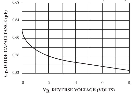
FIGURE 7. CAPACITANCE (BAV99W)
