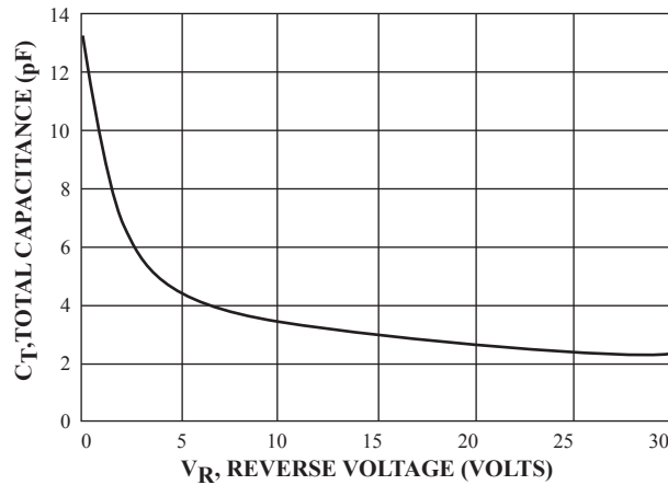
FIG.4 Total Capacitance
