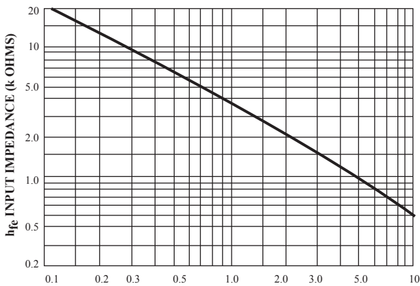
Figure 13. Input Impedance
