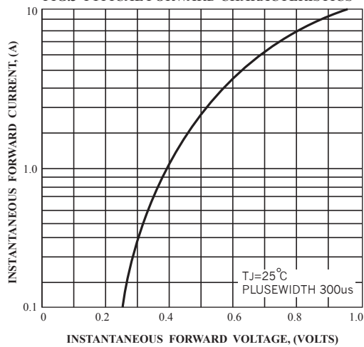
FIG.3-TYPICAL FORWARD CHARACTERISTICS
