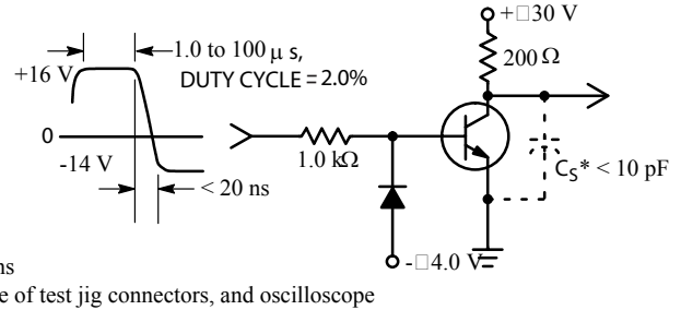
Figure 2. Turn-Off Time
