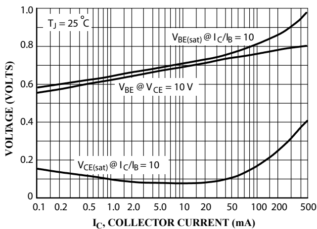
Figure 17. "On" V oltages
